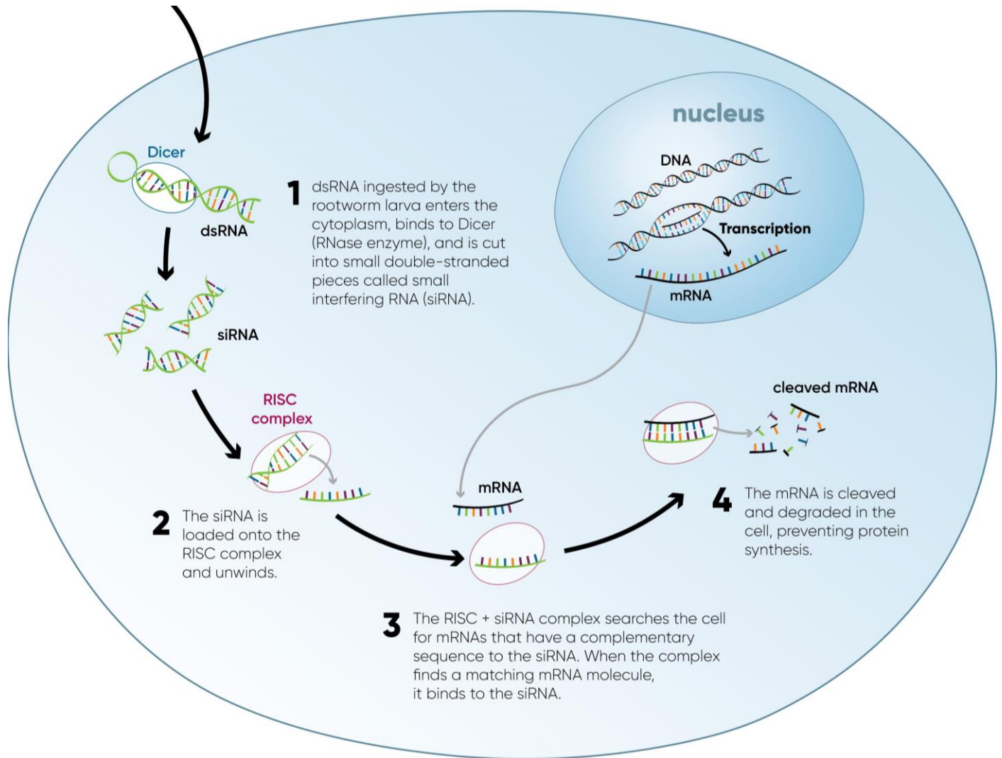
Figure 2. Diagram showing the key steps in the RNAi pathway in a corn rootworm cell. dsRNA produced by the corn plant and ingested by the corn rootworm initiates the RNAi process in the rootworm’s cells, blocking production of a key protein essential for the rootworm’s survival.
